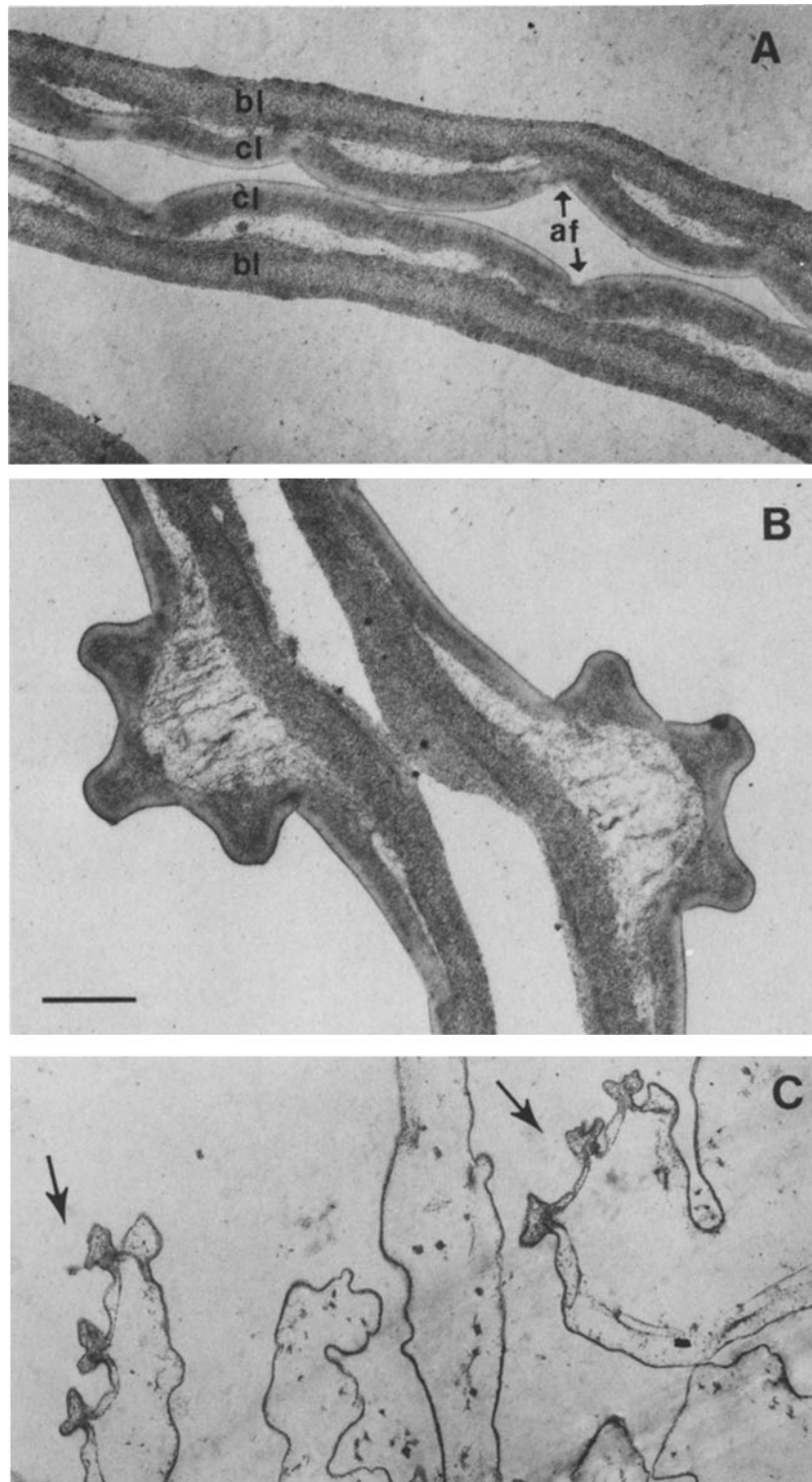
FIGURE 5 Transmission electron micrographs of purified adult cuticles before and after treatment with BME. A and B , SDS-purified cuticles. The three sublayers of the basal layer ( bl ) and varying electron-dense zones of the cortical layer ( cl ) are clearly visible in the cuticles shown in A . Only one of the two fiber layers appears fibrillar in these cuticles, due to the orientation of the section. Annular furrows ( af ) are indicated. B , buckled appearance of the lateral alae after treatment with SDS. Note the fibrillar material underlying the alae. C , cuticle material remaining after treatment with BME. Arrows point to the remains of the lateral alae. All micrographs \times 12,200 . Bar, 1 \mu\text{m} .
